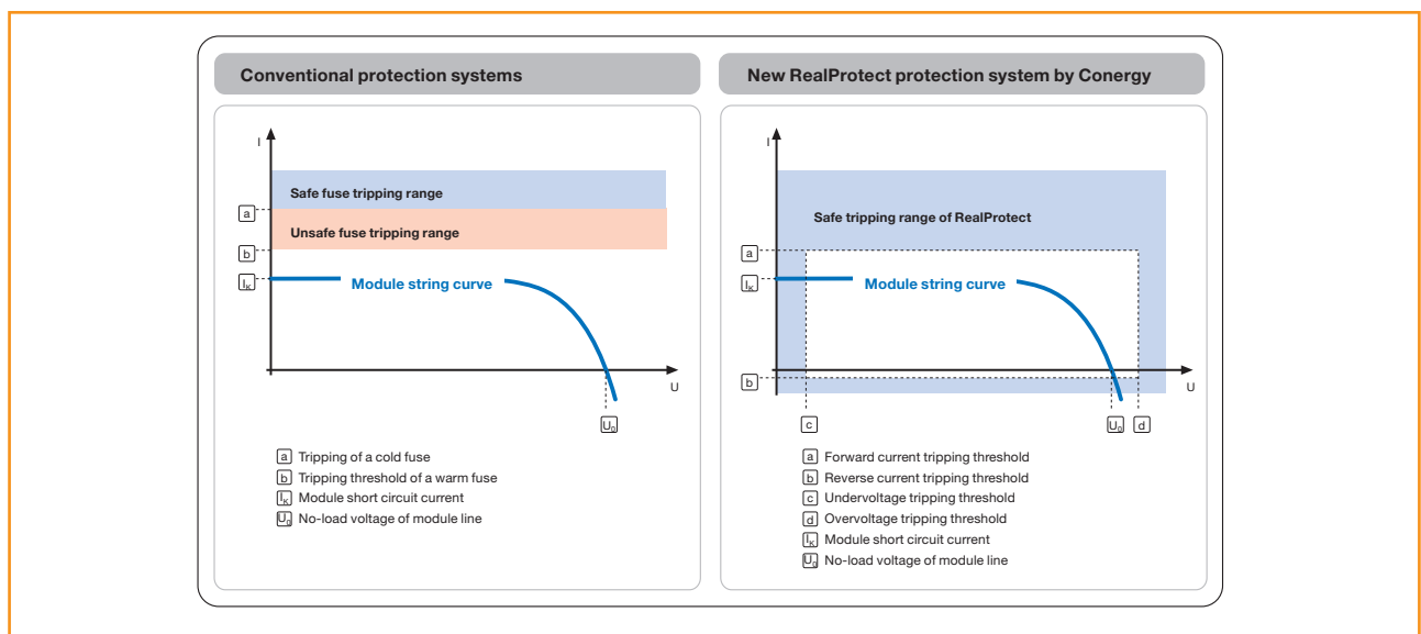
Advantage of the innovative RealProtect protection concept by Conergy
